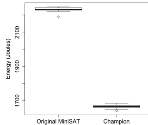
(b) Ensemble
