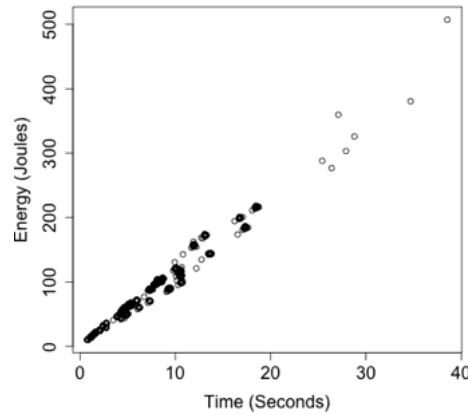
(a) CIT
