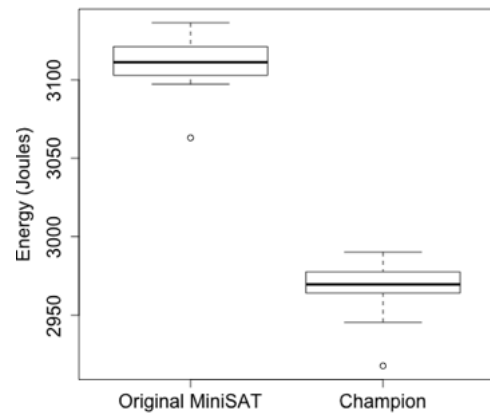
(a) CIT
